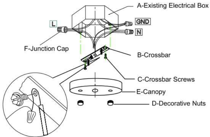
Wire Connection Diagram:
