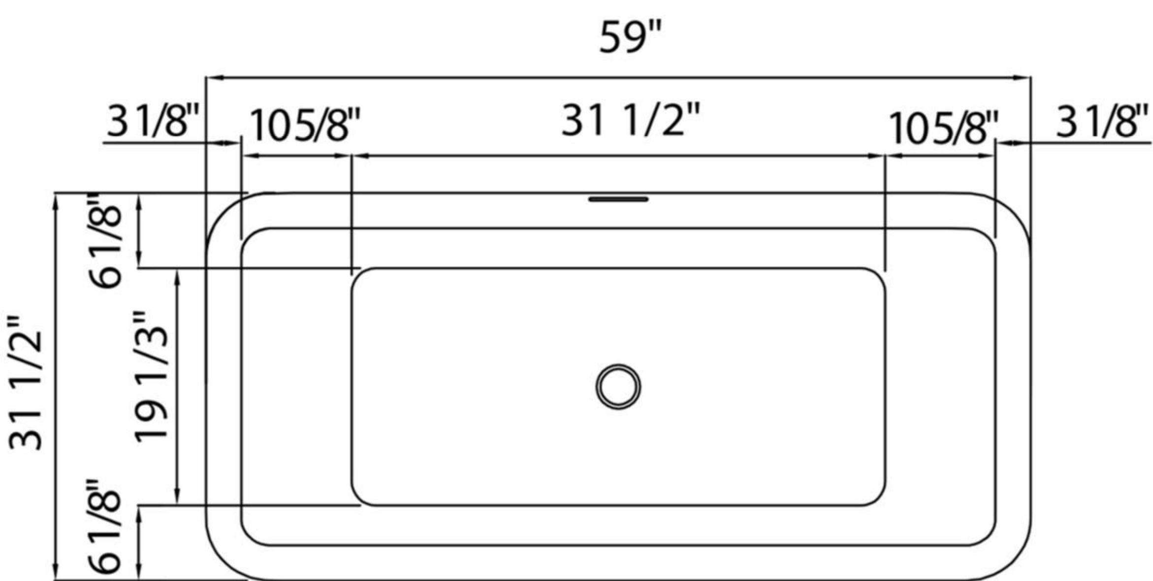
TOP VIEW
