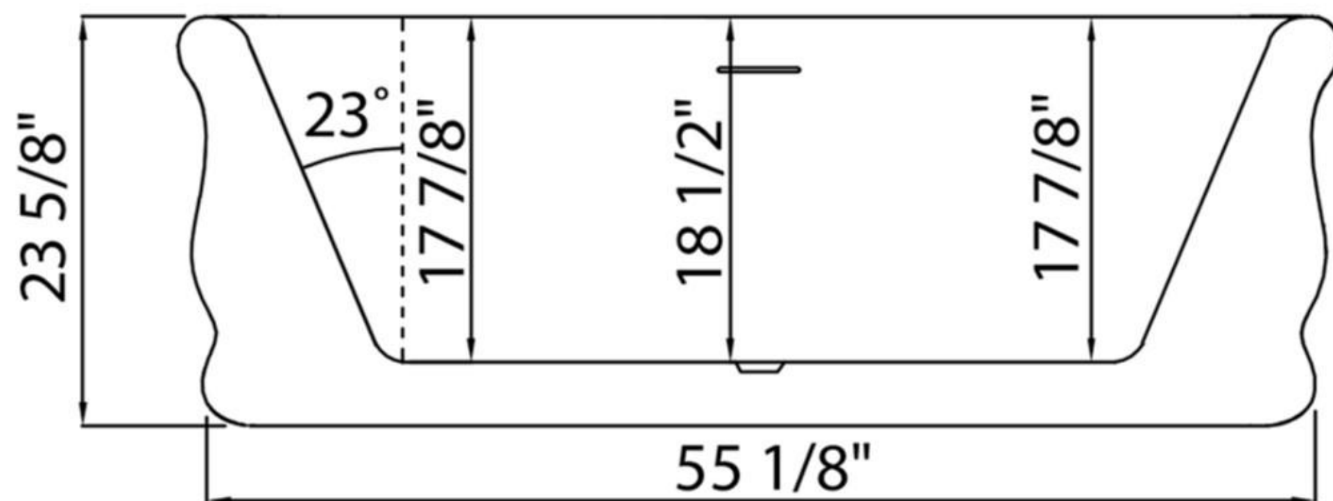
FRONT VIEW
