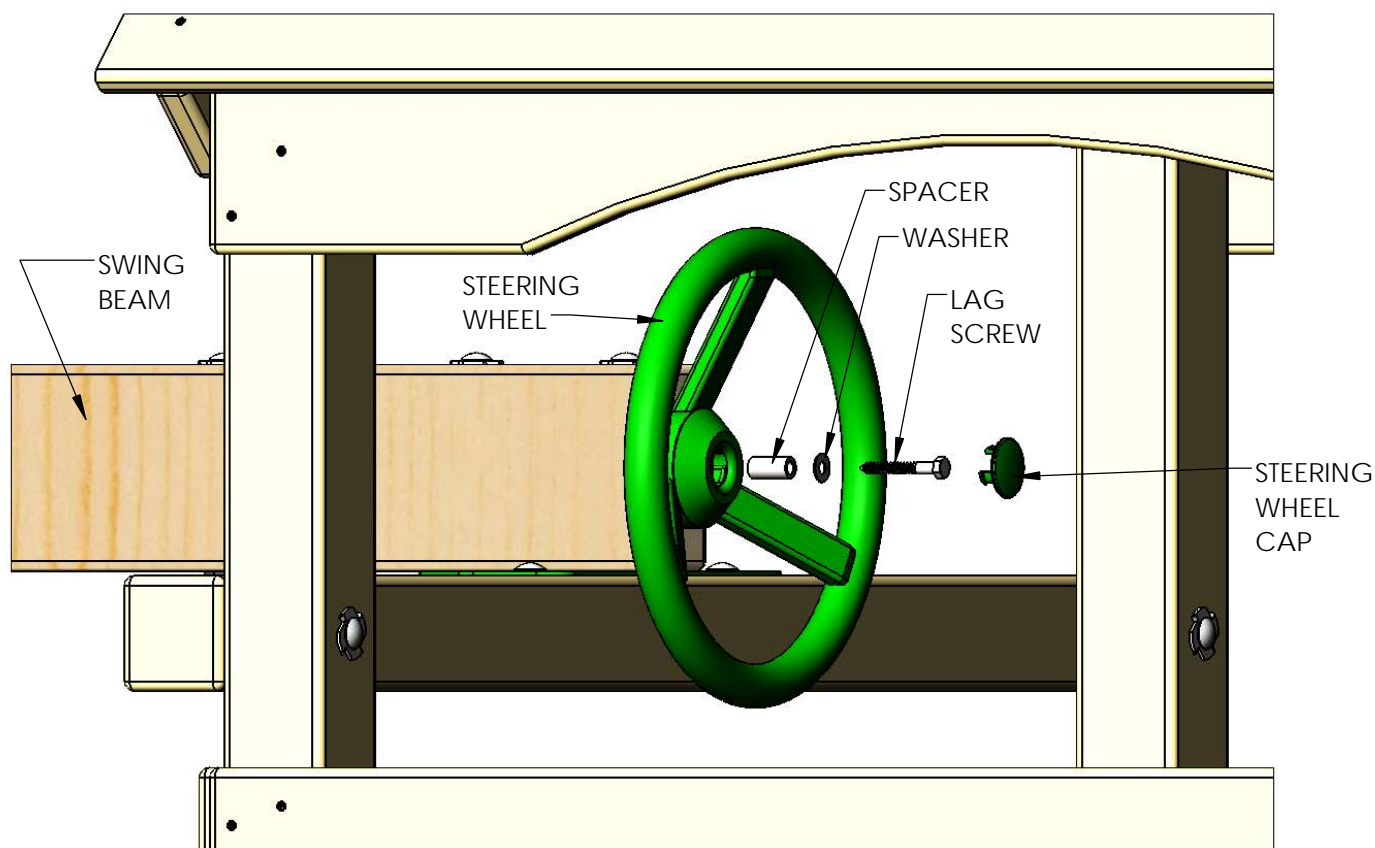
DETAIL A
