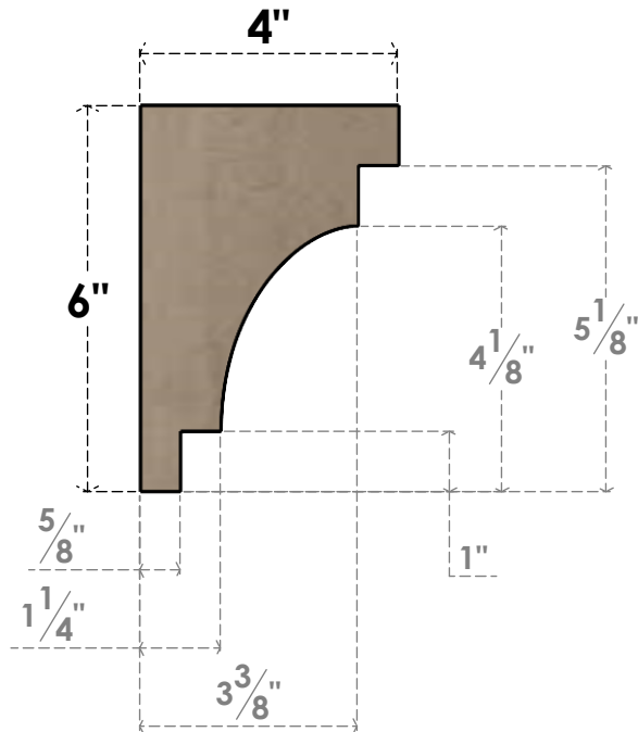
SIDE PROFILE
