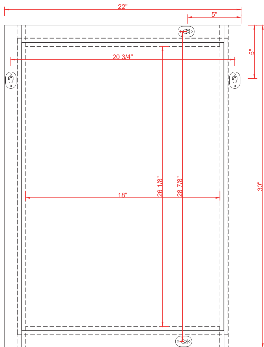
FRONT VIEW
