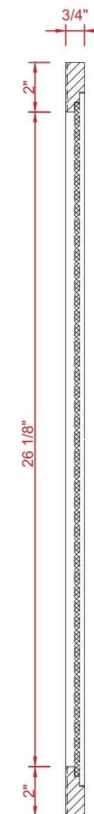
SIDE VIEW
