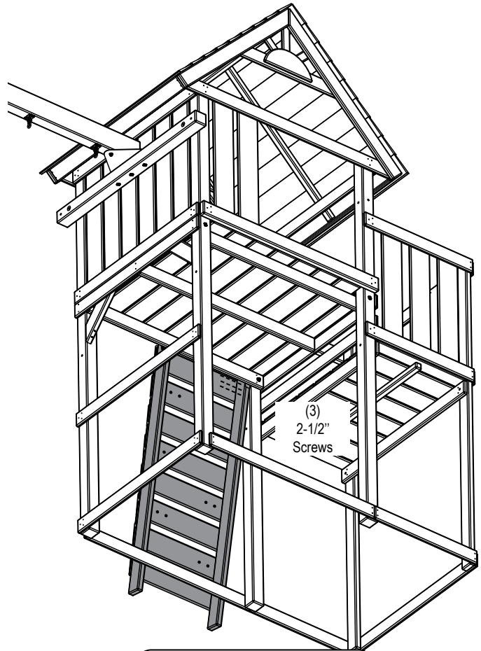
Under Deck View
