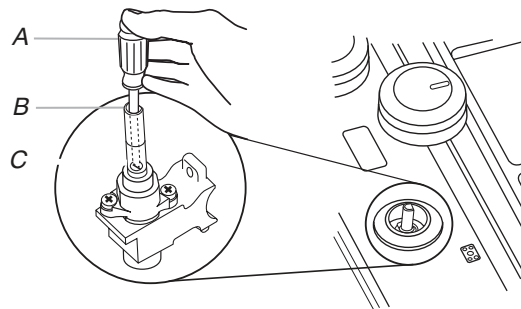
A. \frac{3}{32} " (#0 [2.0 mm]) flat-blade screwdriver (screwdriver shaft must be a minimum of 2" [5.1 cm] long) B. Control knob stem opening C. Adjustment screw location
