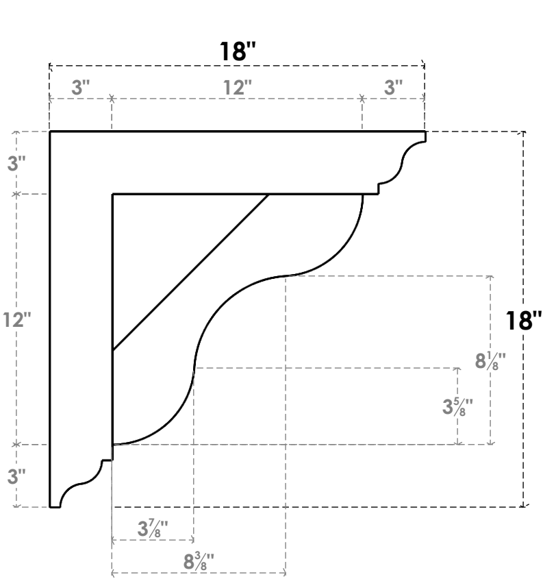
SIDE PROFILE
