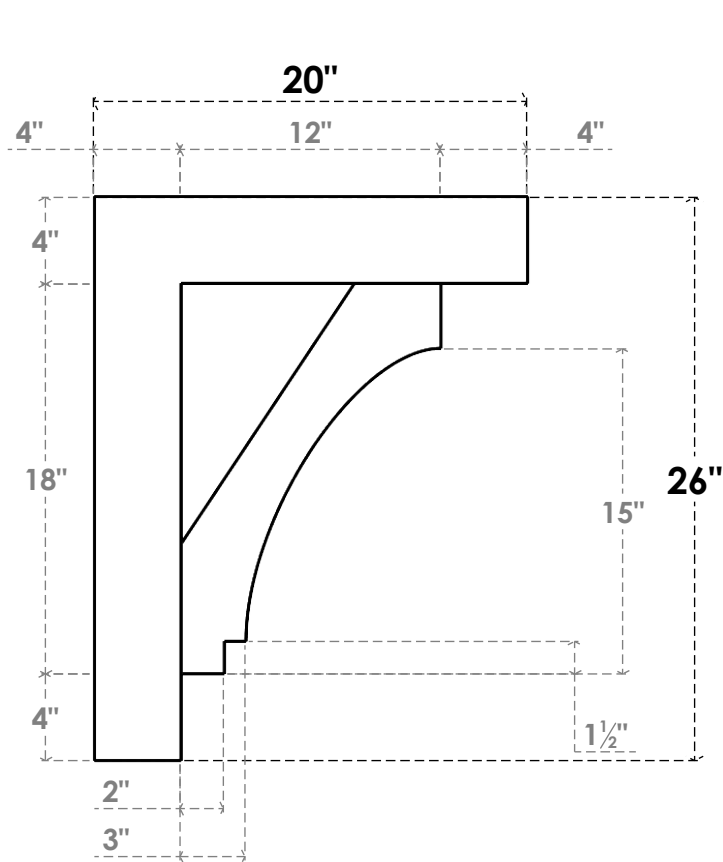
SIDE PROFILE
