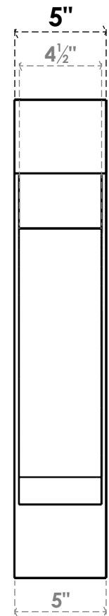
FRONT PROFILE
