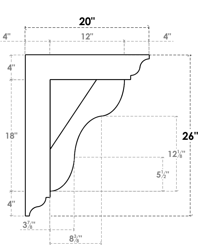
SIDE PROFILE
