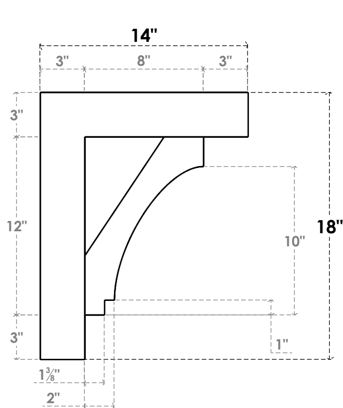
SIDE PROFILE
