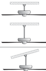
downrod installation
