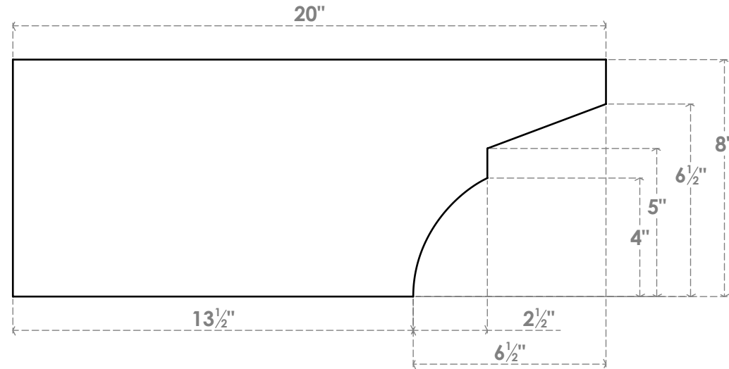
SIDE PROFILE
