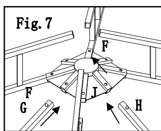
Fig.7: Insert Middle beam(G/H) to Big top connector(J).
