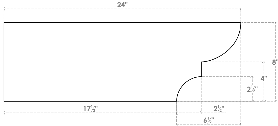
SIDE PROFILE
