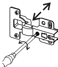
Lateral adjustment
