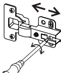
Depth adjustment
