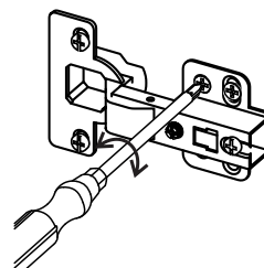
Front screws adjustment
