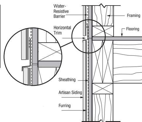
Figure 13 Bridging Floors
