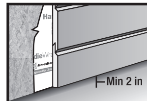
Figure 9 Mortar/Masonry
