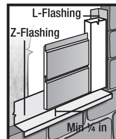
Figure 9 Mortar/Masonry
