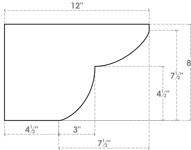
SIDE PROFILE
