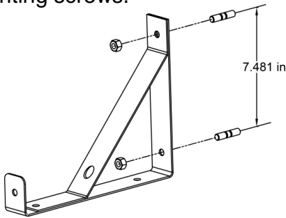
WALL MOUNT
