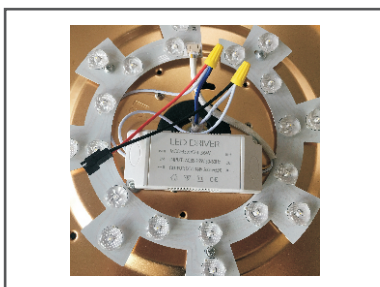
Step 3. Wiring diagram of LED light source and LED driver and Bluetooth connection cable.
