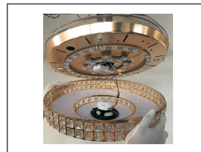
Step 6. Connect the Bluetooth drive cable on the lampshade with the Bluetooth cable on the chassis of the fan lamp host.
