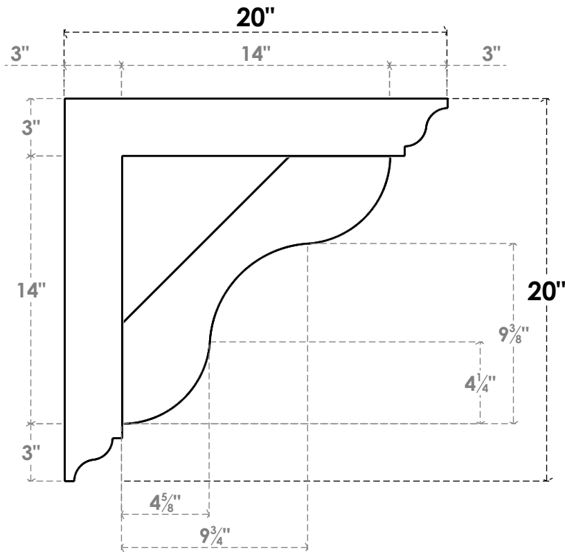
SIDE PROFILE
