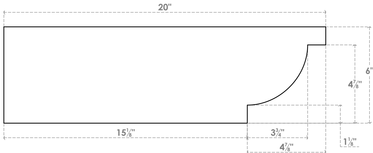
SIDE PROFILE
