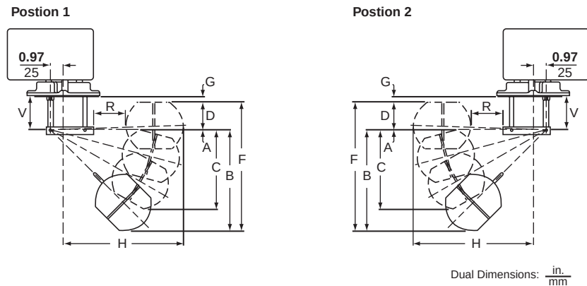
Figure 23: Travel Dimensions
