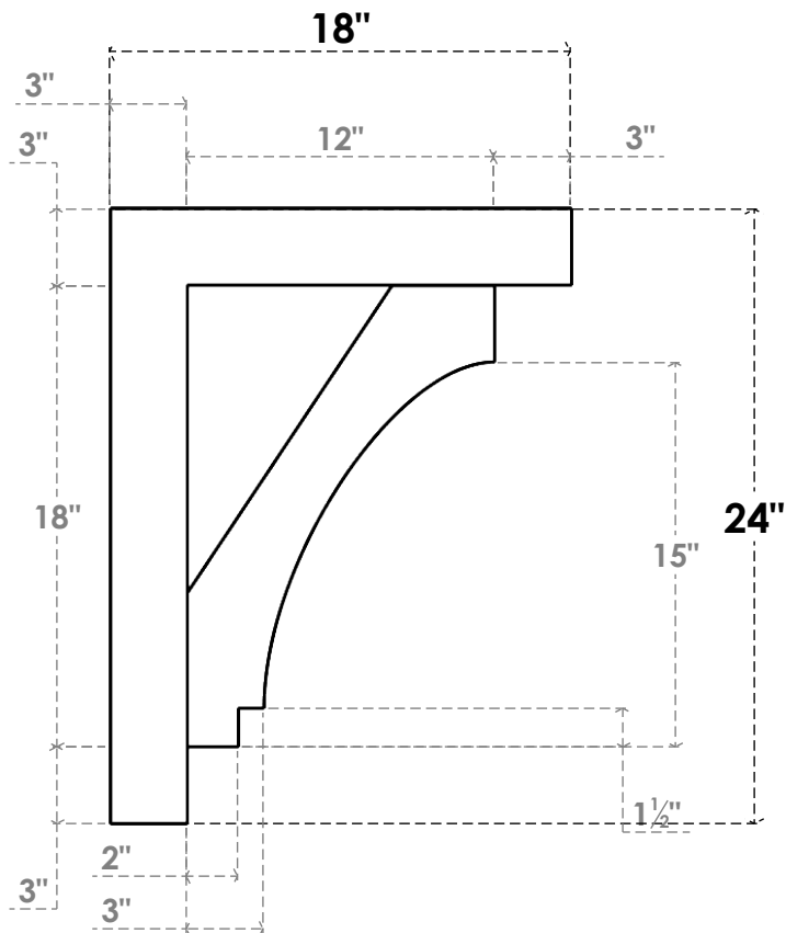
SIDE PROFILE
