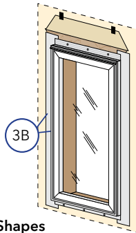
Building Wrap Cutting Patterns for Window Shapes
