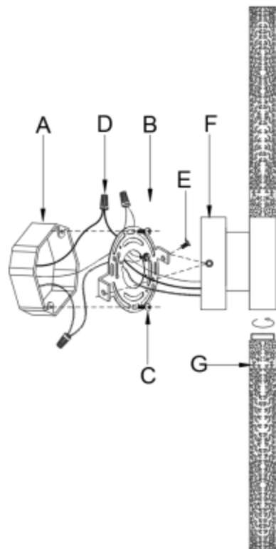
After securing fixture to the wall it is recommended that the gap between the wall and the fixture backplate be sealed on the top and both sides, with a good quality waterproof caulk or silicone sealant (NOT INCLUDED)-see Drawing 1.
