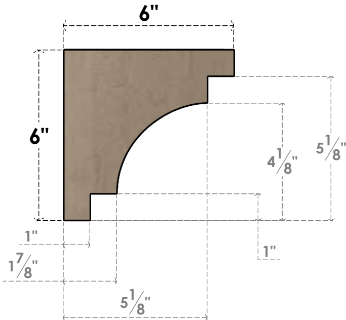
SIDE PROFILE
