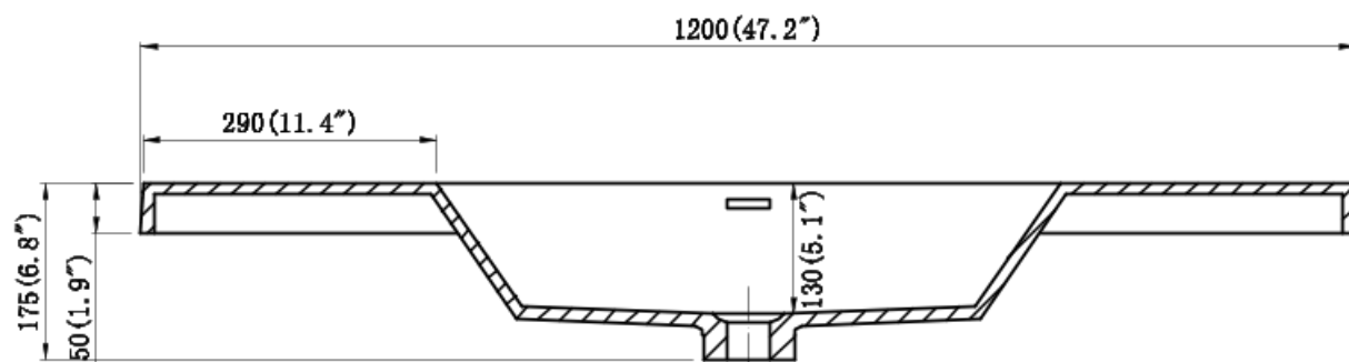
SECTION B-B
