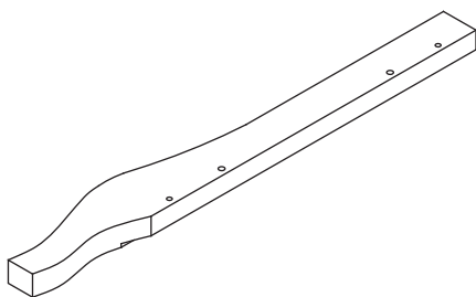
3 Back Leg (Left) Qty 1 (25.39×2.75×0.98")
