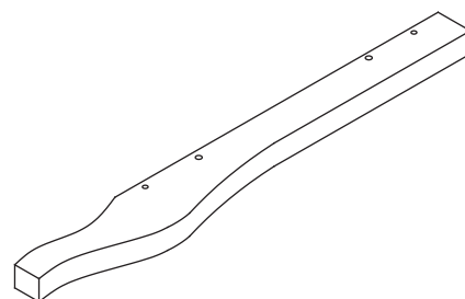
2 Front Leg (Left) Qty 1 (25.39×2.75×0.98")
