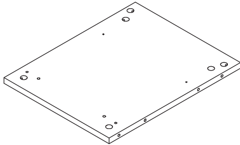
7 Side Panel (Right) Qty 1 (10.62×15.55×0.47")
