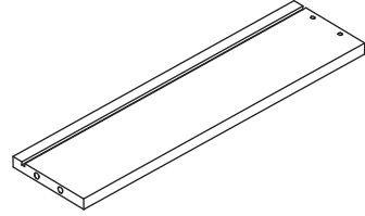
14 Drawer Side (Right) Qty 1 (11.81×3.93×0.47")
