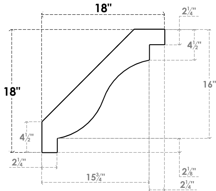
SIDE PROFILE
