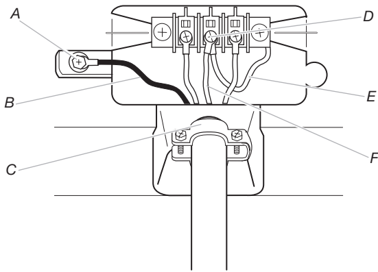
A. External ground conductor screw B. Ground wire (green or bare) of power supply cord C. 3/4" (19 mm) UL listed strain relief D. Center terminal block screw E. Neutral ground wire F. Neutral wire (white or center wire)
