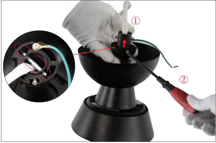
Step 7 1. Push the hemisphere upward. 2. Tighten the screw on the hemisphere.
