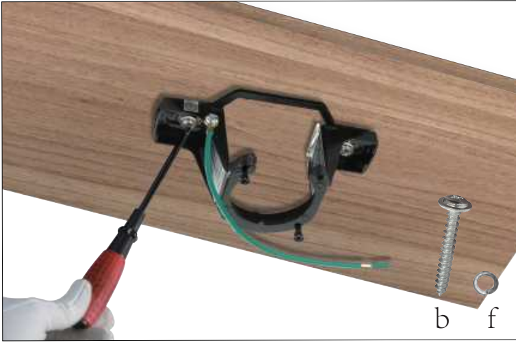
Step 1 For wooden ceiling, install the Hanging bracket to Wooden ceiling with two wood screws.
