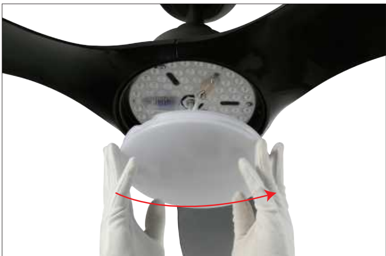
Step 16 Rotate the light cover until fixed.
