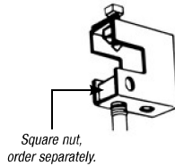
U562 Beam Clamp Optional Use 1/2" set screw included. Rod size: 1/2" Design load 800 lbs. For 20° swivel application, use ES-145-1/2 nut.
