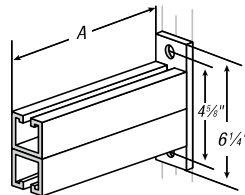
S-251 Strut section made from half slot channel. Sizes: 12", 18", 24", 30" & 36"
