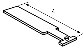
U-568 Beam Clamp Safety Strap Standard Finish — GoldGalv® brand For U-563 beam clamp.
