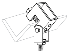
US562 Beam Clamp with Swing Hanger 1/2" screw included. Rod size: 1/2" Design load 800 lbs.
