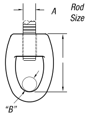
M-117 MI Socket only for S Split Ring Hanger Sizes ¾" through 1½" rod Federal Type 16 SP69 Type 16
