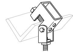
U563 Beam Clamp with Swing Hanger 3/8" set screw included. Rod sizes: 3/8" Design load 540 lbs.
