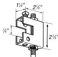
U562 Beam Clamp 1/2" set screw included. Rod Size: 1/2" Design load 500 lbs.
