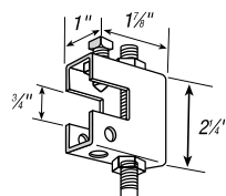
U563 Beam Clamp 3/8" set screw included. Rod size: 3/8" Design load 250 lbs.
