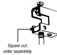
U563 Beam Clamp Optional Use 3/8" set screw included. Rod size: 3/8" Design load 400 lbs.
