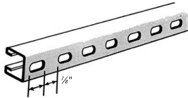
A-1200-HS_AL Slots 2" on center. Slot size 7/16" x 1 1/8"
