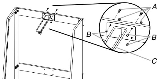
A. Phillips-head screws (F3b) B. Acorn nuts (F10) C. Golf bag divider
