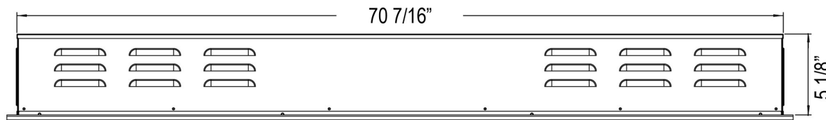
Top View
