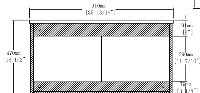
Back View
