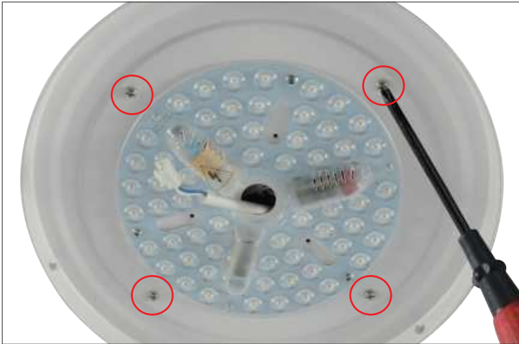
Step 18 Fix the light plate with the screws.
