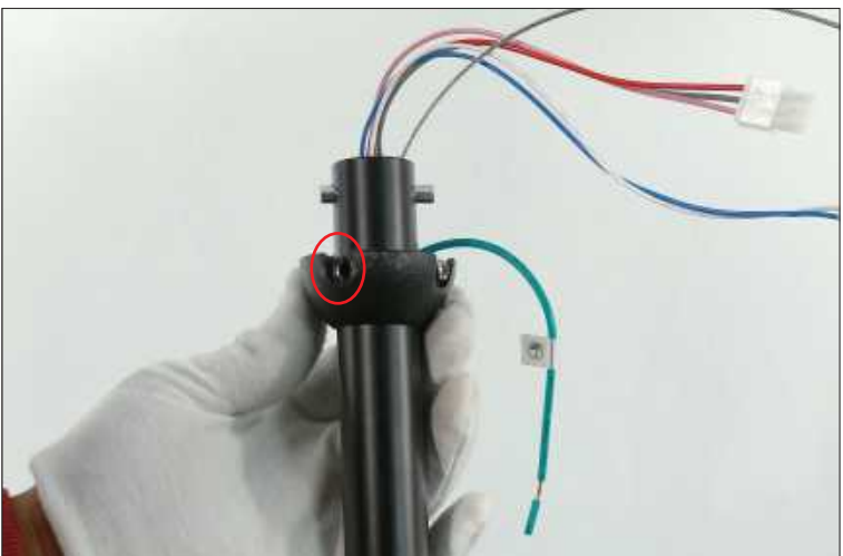
Step 9 Push the hemisphere up, Align the small rod with the notch on the hemisphere
