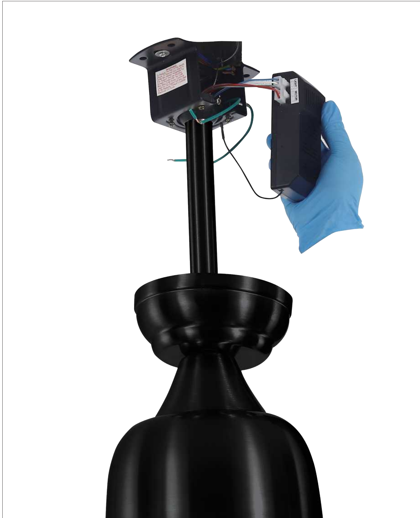
Step 12 Connect the wires from motor to receiver.
