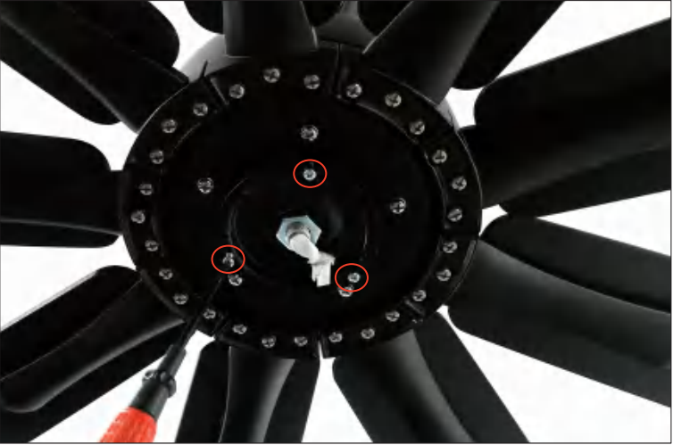
Step 18 Remove the three screws which are used to install the light kit.
