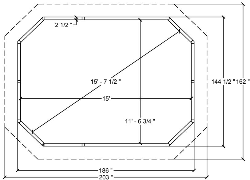
PLAN A LA BASE PLAN AT THE BASE
