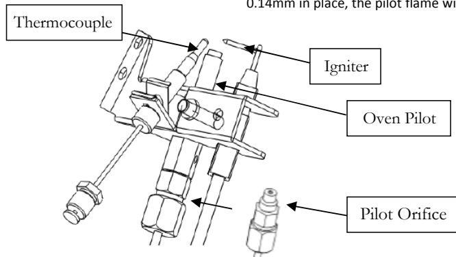
Pilot Orifice
