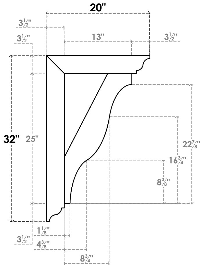
SIDE PROFILE
