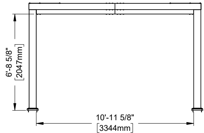
16' X 12' MODERN METAL PERGOLA FOOTPRINT
