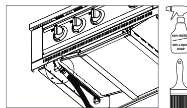
Leak Testing Diagram
