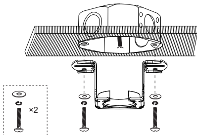
Outlet Box
