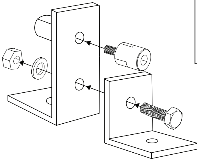
Spacer Connector (1)
