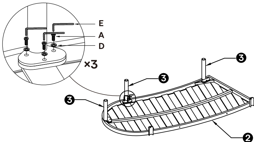
3 Legs ③ + 1 Seat Frame ②+ Hardware package
