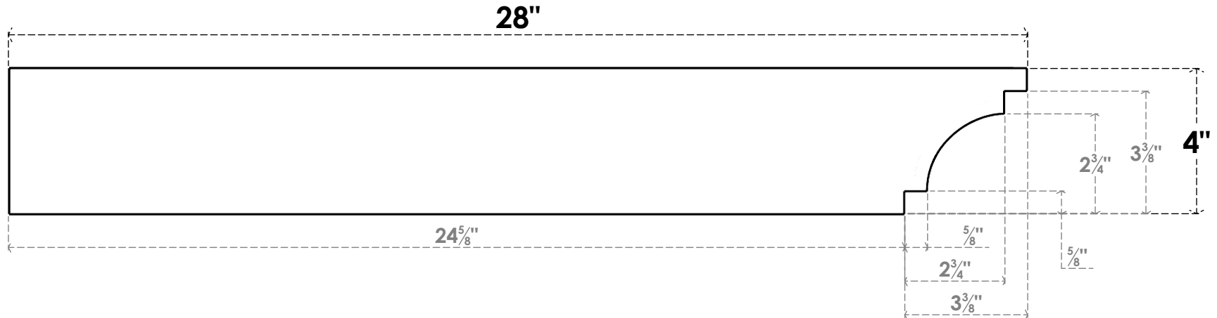
SIDE PROFILE
