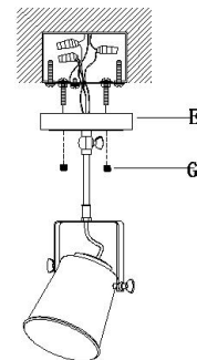
CEILING & OUTLET BOX
