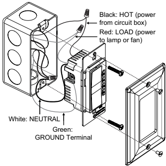
Fig. 3. Switch Orientation, Wires Connections and Wall Box Assembly
