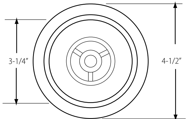
Sink Body
